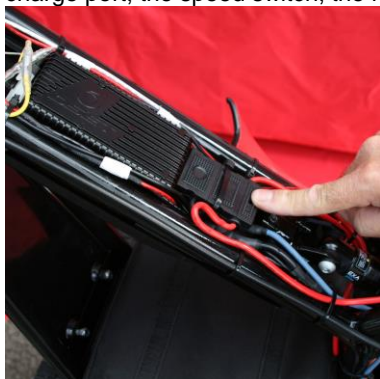
Controller and fuse.
